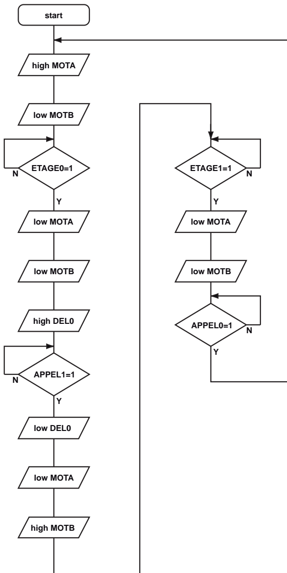
Programme Monte Charge 3.cad
