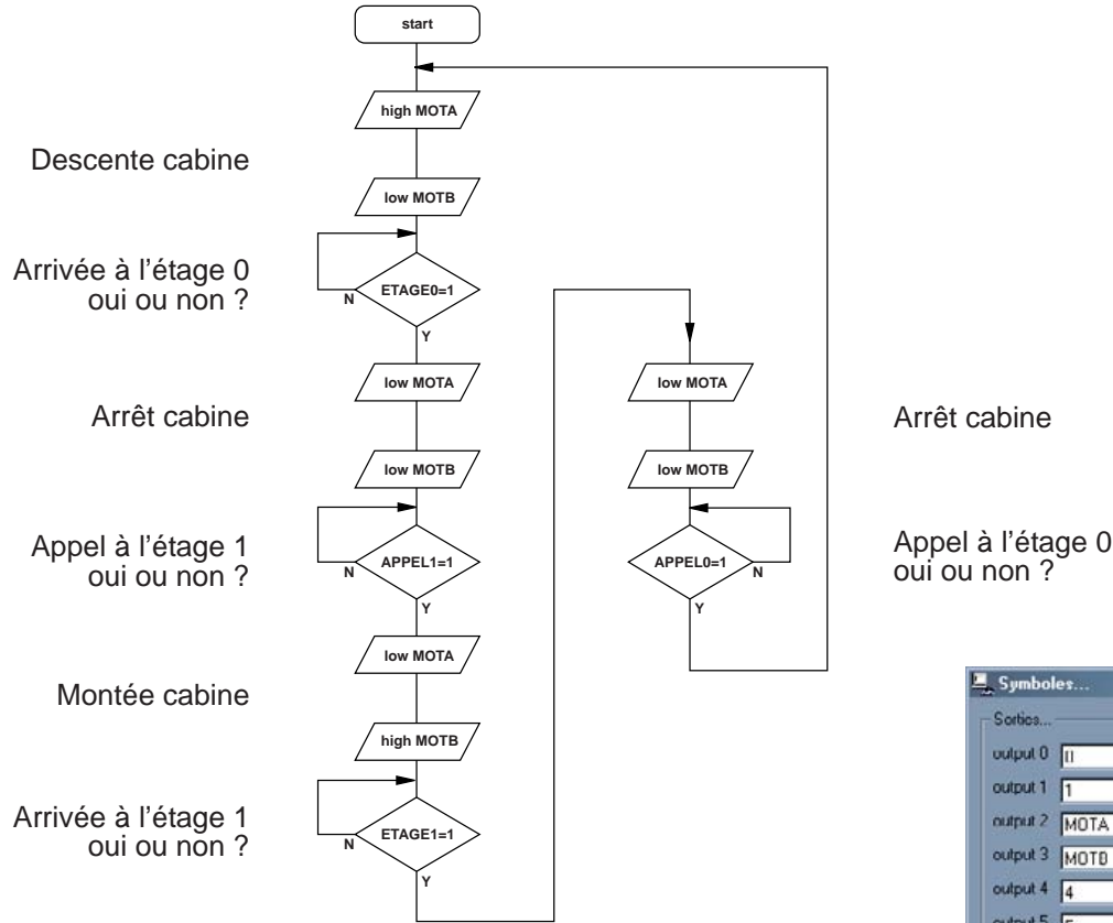
Programme "Monte Charge 1.cad"
