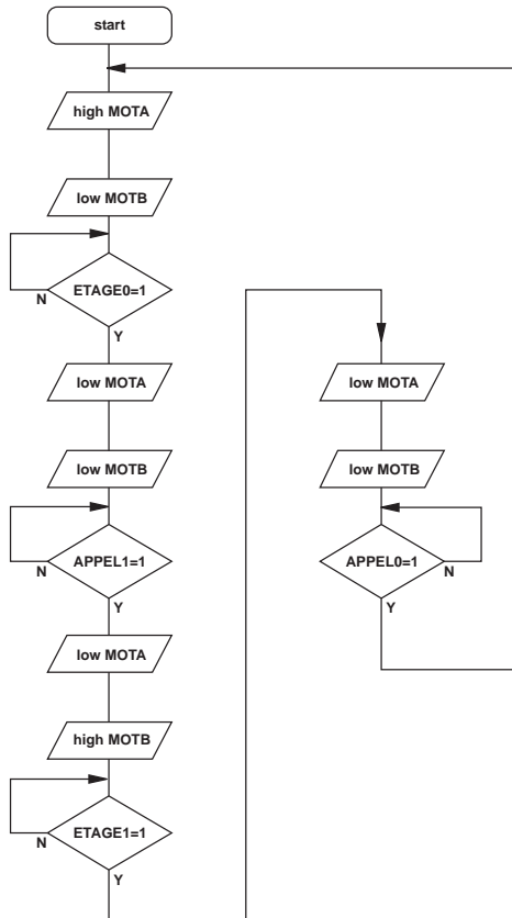
Programme "Monte Charge 1.cad"
