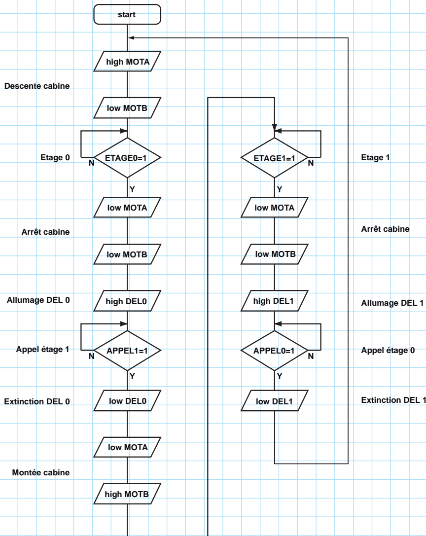
Programme Monte Charge 3.cad
